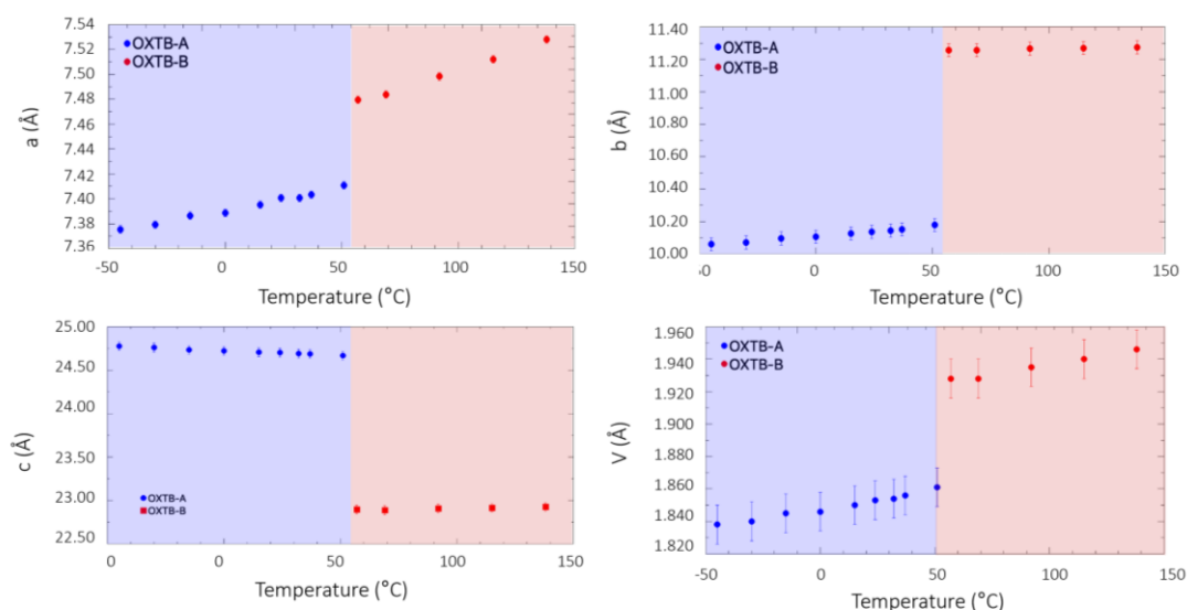
Figure 34 Unit cell parameters of oxitropium bromide as a function of temperature determined by in-situ high-temperature powder X-ray diffraction from -45°C – 15°C and in-situ high-temperature single crystal X-ray diffraction 24°C – 138°C. Blue and red rectangles.
