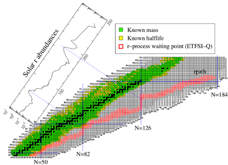
Figure 1.5: Illustration of r-process paths (red squares) and the observed r-process abundances (inset). Blue solid lines indicate proton and neutron magic numbers. From Ref. [39].
