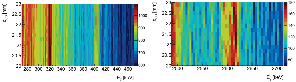
Figure 3.3: The d_{CD} vs. E_\gamma matrix in the selected energy ranges, obtained with the use of 1 mg/cm 2 target. Left: Doppler corrected for light fragment. Right: Doppler corrected for heavy fragment. Notice the difference in the binning.
