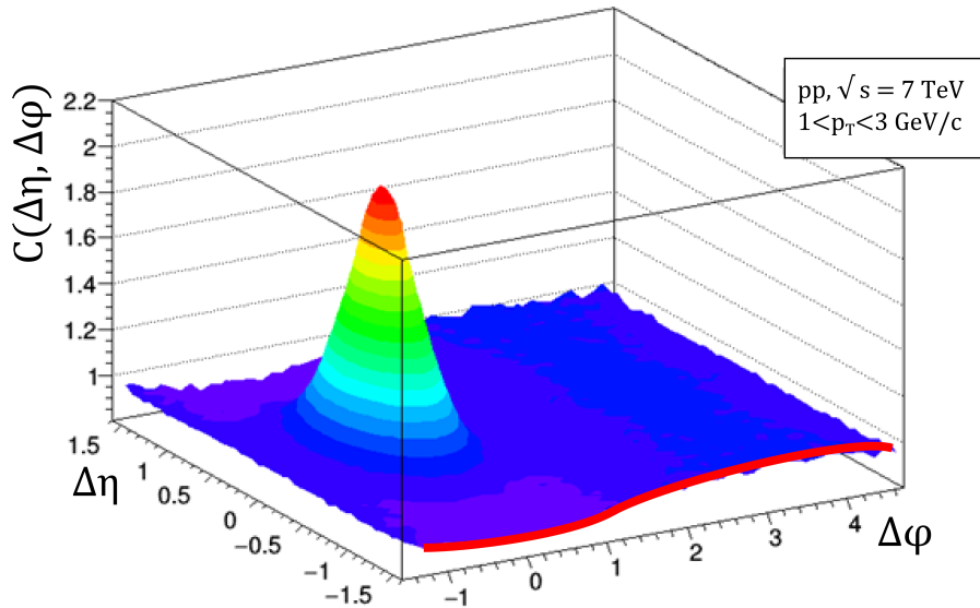
Figure 3.7: Momentum conservation contribution to the correlation function C(\Delta\eta, \Delta\varphi) (marked in red).
