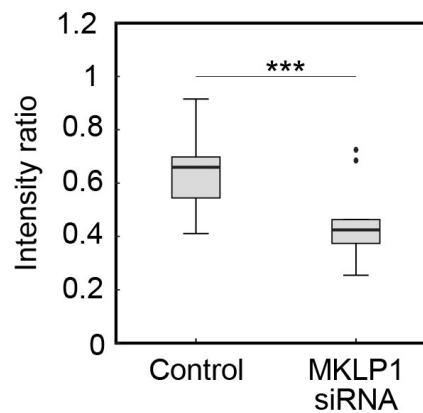
Figure 62 MKLP1 depletion affects the midzone stability. (a) Smoothed time-lapse images (left panel) of the anaphase spindle after photoactivation of PA-GFP-tubulin at time of photoactivation (0s) and after photoactivation (60s) in the bridging fibers in MKLP1 depleted spindles (top row) and control spindles (bottom row). Signal intensity of PA-GFP-tubulin (right panel), measured across the midzone, at time of photoactivation (0s) and after photoactivation (60s) in the bridging fibers in MKLP1 depleted spindles (top row) and control spindles (bottom row). (b) Box plot of signal intensity ratio (signal in the midzone 60s after photoactivation/signal in the midzone at time of photoactivation) for the conditions from a).
