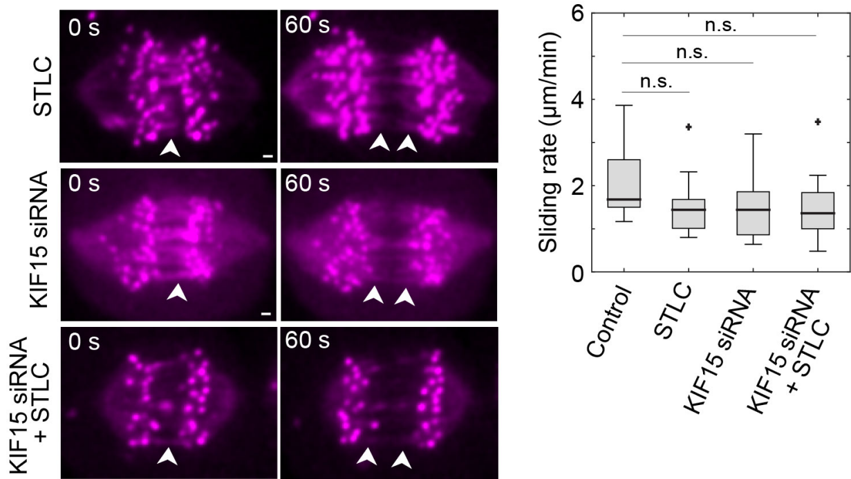
Figure 60 Depletion of Eg5 and KIF15 does not affect sliding velocity. Smoothed time-lapse images (left panel) of the anaphase spindle after photoactivation of PA-GFP-tubulin at time of photoactivation (0s) and after photoactivation (60s) in the bridging fibers in STLC treated spindles (top row), KIF15 depleted spindles (middle row), Kif15 depleted and STLC treated spindles (bottom row). White arrowheads mark the photoactivated spot, which splits into two spots. Box plot (right panel) of sliding rates for control spindles and for the conditions from. n.s. non-significant.
