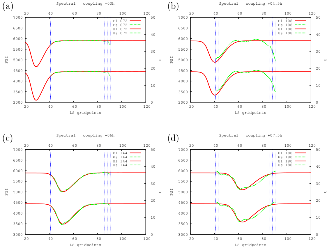
Figure 4.10: Results using spectral coupling scheme with 3 h interval between input large scale data, when amplitude and phase are interpolated in time using the extrapolated values after 3 (a), 4.5 (b), 6 (c) and 7.5 (d) h. Lines have the same meaning as in Fig. 4.1. The numbers in the legend are the number of forecast time steps. The vertical axes are geopotential in gpm and wind variable in m/s.
