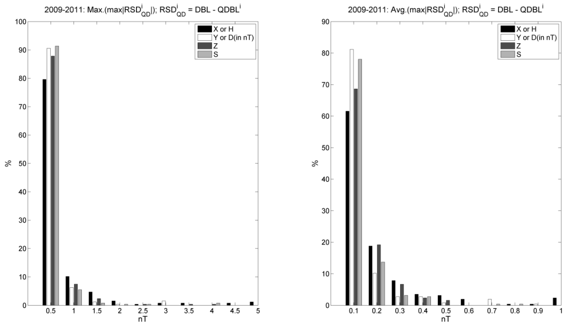
Figure 4.4 Left: Annual maxima of the maximal residuals between the new DBL and its temporary baseline segments (QDBL), i.e. each maximal residual correspond to one baseline window. Right: Annual averages of the same residuals presented in the left subplot.
