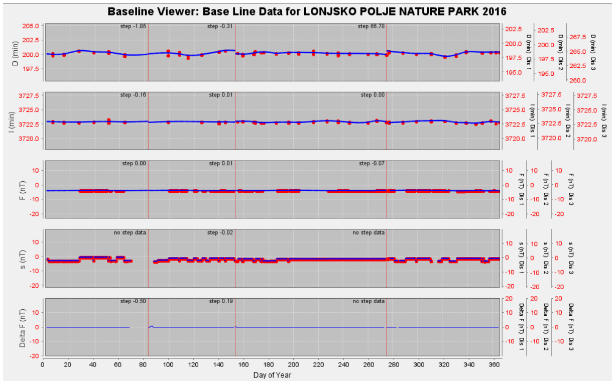
Figure 2.5 The dIdD baselines for the year 2016 at LON geomagnetic observatory. Observed baselines obtained from absolute measurements are presented by red dots. Continuous functions are fitted on the observed values to obtain adapted baselines (blue lines). The vertical red lines indicate the steps in the baseline. The baseline plot is created using IMCDVIEW software.
