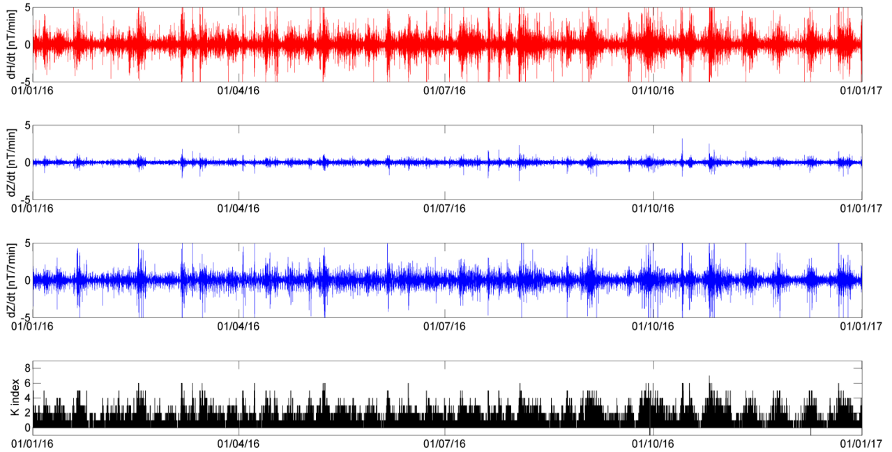
Figure 5.2 Rate of change dB/dt for H and Z components of LON time series during 2016 (see text for details). In the first and third subplots at some periods (enhanced geomagnetic activity), values exceed \pm 5 nT. The ordinate scaling of \pm 5 nT is used for better visibility. The bottom subplot displays local geomagnetic indices during 2016.
