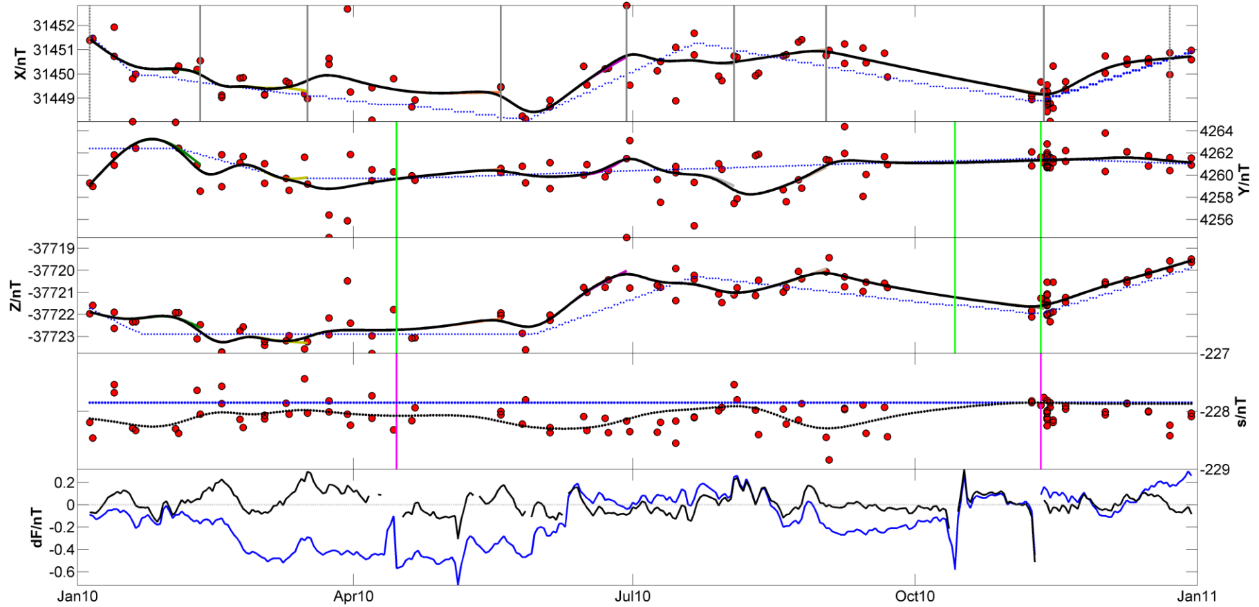
Figure B1.1. Green vertical lines show three discontinuities in vector baselines (only second and third diagram). Two discontinuities in scalar baseline are presented by magenta vertical lines. Generally, the number of discontinuities in vector and scalar baselines is different.
