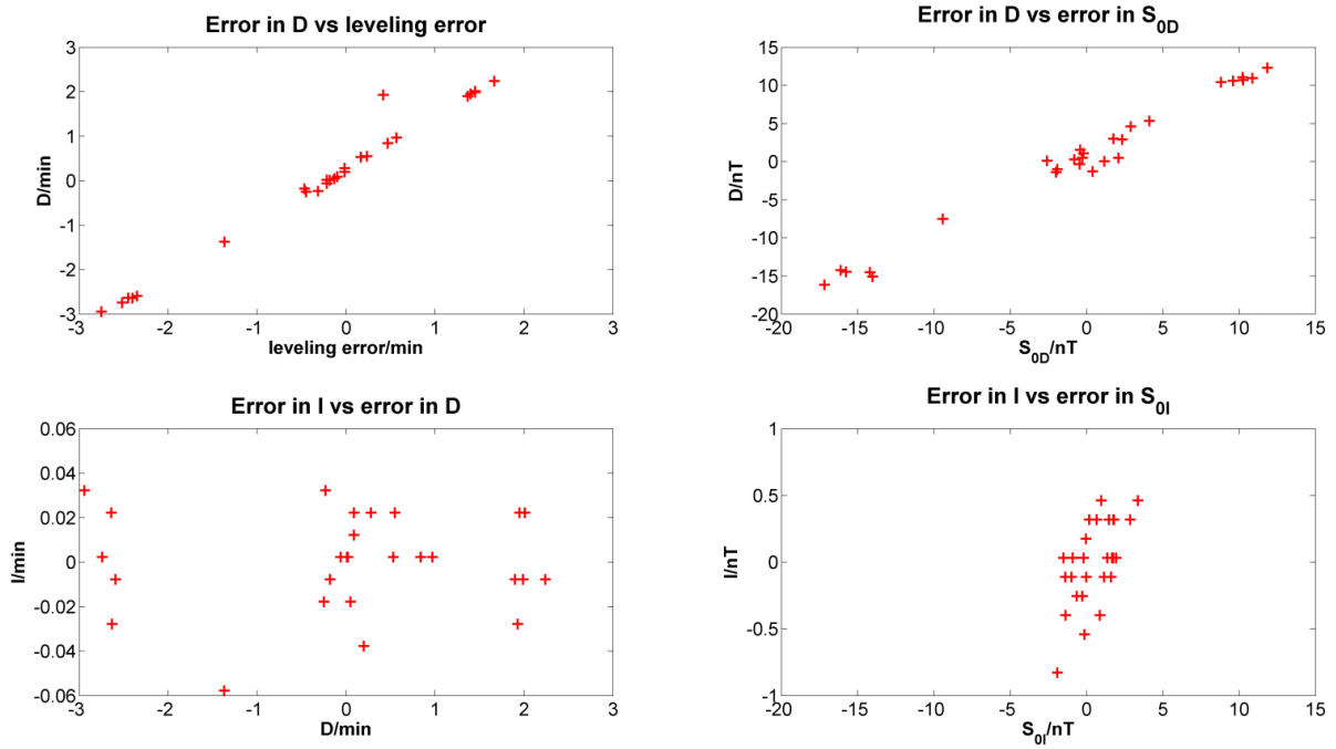
Figure 2.6 Results of test measurements performed at Niemegk observatory during May and June 2014. Top-left: Errors in D caused by improper levelling. Top-right: Errors in S_{0D} parameter are also linked with levelling errors. Bottom-left: Errors in I versus errors in D , i.e. error in setting the telescope in the magnetic meridian. Bottom-right: Errors in I versus errors in S_{0I} parameter. Note that D and I (arc minutes) on the left subplots are expressed in equivalent units in nT on the right subplots.
