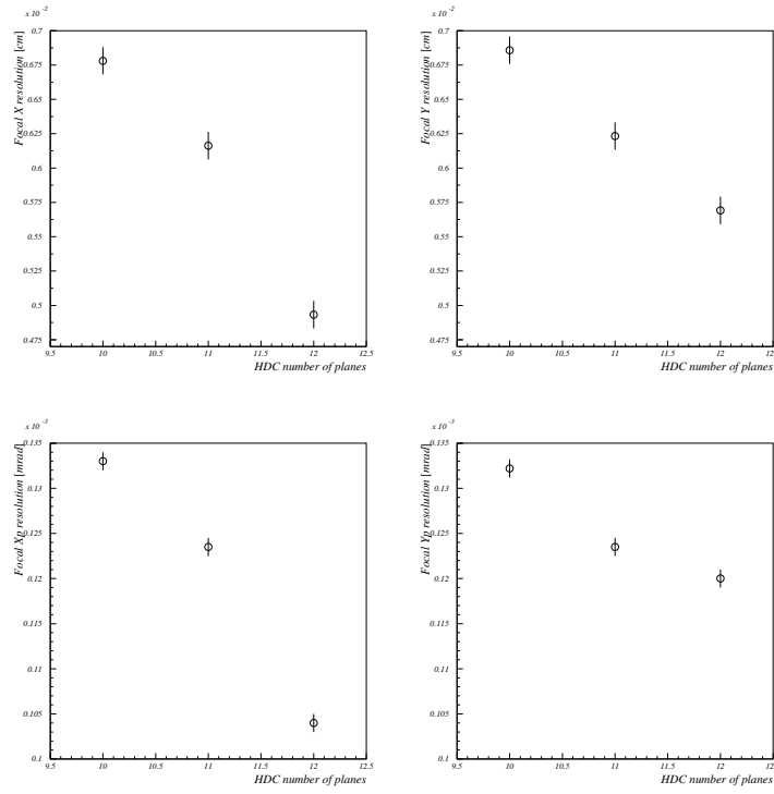
FIGURE 4.35: AVERAGE RESOLUTION OF HKS FOCAL PLANE QUANTITIES AS A FUNCTION OF THE NUMBER OF HDC PLANES USED IN TRACKING ALGORITHM. ANALYSIS WAS DONE FOR \text{CH}_2 DATA AND RESOLUTION IS DEFINED AS SIGMA OF THE GAUSSIAN.
