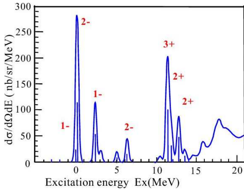
FIGURE 5.7: CALCULATED SPECTRUM FOR THE ^{12}C(e, e'K^+)^{12}_{\Lambda}B REACTION AT E_{\gamma} = 1.3 GeV AND \theta_{K^+}^{LAB} = 3^{\circ} WITH FIXED ENERGY RESOLUTION OF 300keV (FWHM). UPDATE WITH NSC97F FROM [94] [95].
