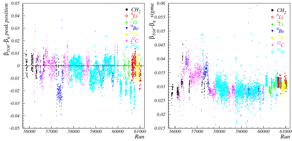
FIGURE 3.12: Left \Delta\beta_{\Pi} PEAK CENTER VALUE AS A FUNCTION OF RUN NUMBER. Right \Delta\beta_{\Pi} RESOLUTION (GAUSS \sigma ) AS A FUNCTION OF RUN NUMBER.
