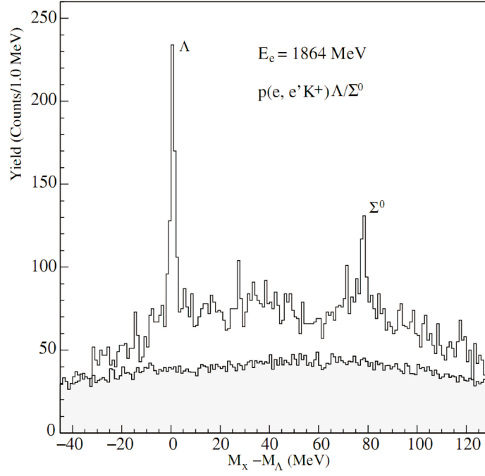
(a) Missing mass spectra from \text{CH}_2 target
