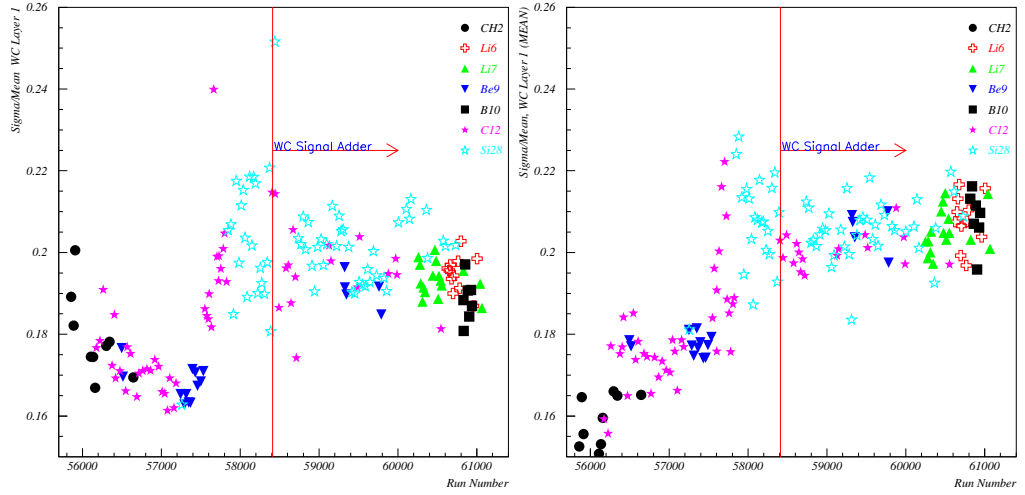
FIGURE 3.34: QUOTIENT OF SIGMA AND MEAN OF PHOTOELECTRONS DISTRIBUTION IN WC LAYERS. THE MEAN (SIGMA) VALUE CORRESPONDS TO THE MEAN (SIGMA) OF THE GAUSSIAN FIT OF THE KAON EVENTS.
