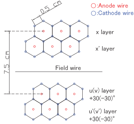
FIGURE 2.23: HONEYCOMB CELL STRUCTURE OF THE ENGE DRIFT CHAMBER.
