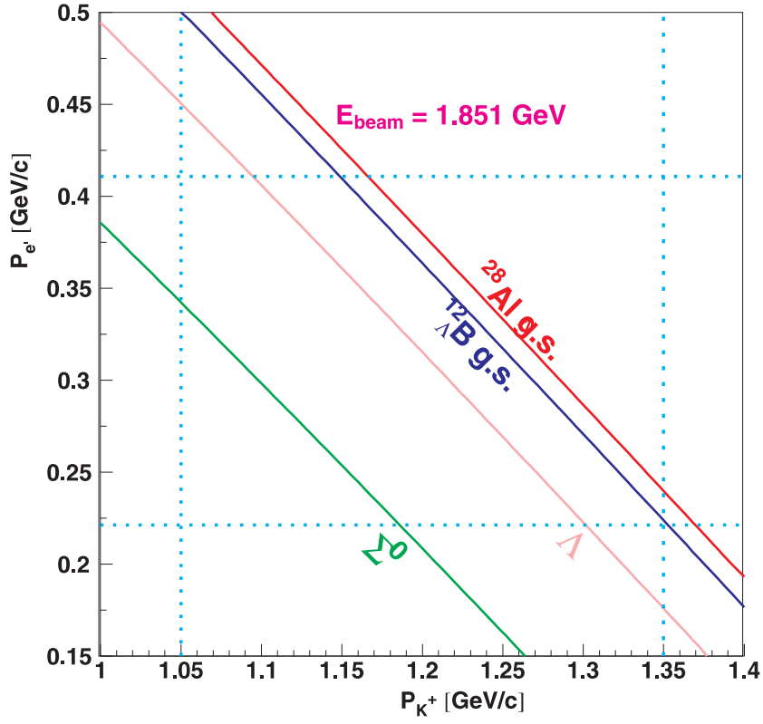
FIGURE 2.3: MOMENTUM ACCEPTANCE OF KAON AND SCATTERED ELECTRON SPECTROMETERS. ( It is calculated with: BEAM ENERGY 1.851 GeV, ASSUMED BINDING ENERGY OF ^{12}_{\Lambda}\text{B} GROUND STATES -11.37 MeV [82] AND ^{28}_{\Lambda}\text{Al} GROUND STATE -16.92 MeV [58].)
