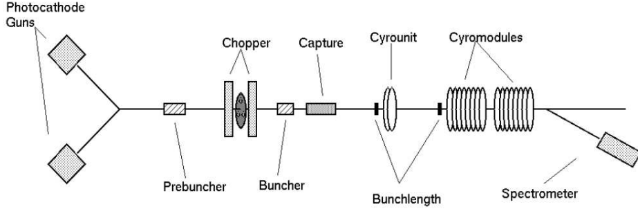
FIGURE 2.7: THE INJECTOR SYSTEM LAYOUT.
