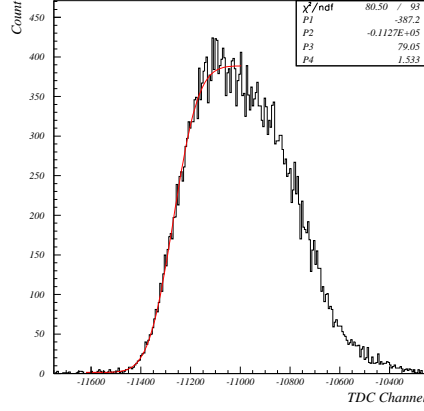
FIGURE 3.8: TYPICAL EDC DRIFT TIME DISTRIBUTION FROM CH 2 DATA. DRIFT TIME WAS USED IN TIME-TO-DISTANCE MAP CALIBRATION.
