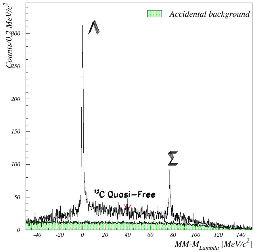
FIGURE 4.23: MISSING MASS SPECTRA FROM \text{CH}_2 DATA. \Lambda AND \Sigma PEAKS ARE CLEARLY SEEN. ACCIDENTAL COINCIDENCES AND QUASI-FREE CONTRIBUTION FROM ^{12}\text{C} ARE ALSO SHOWN.
