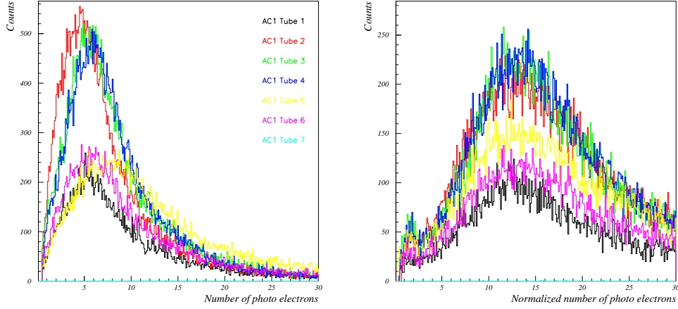
FIGURE 4.6: REAL \text{LI}_7 DATA AEROGEL ČERENKOV NUMBER OF PHOTOELECTRONS DISTRIBUTIONS FOR ALL AC1 LAYER TUBES. Left REAL DATA DISTRIBUTIONS. Right DISTRIBUTIONS AFTER TUBE NORMALIZATION.
