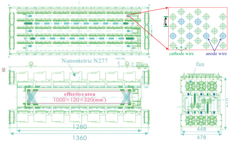
FIGURE 2.24: SCHEMATIC VIEW OF THE ENGE HONEYCOMB DRIFT CHAMBER.
