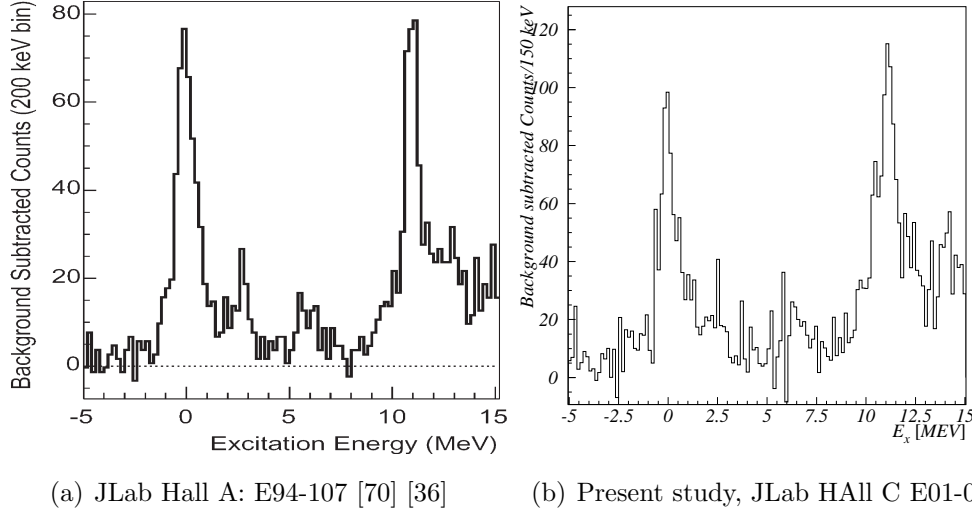
FIGURE 5.6: COMPARISON BETWEEN JLAB HALL A: E94-107 AND HALL C: E01-011 MEASURED ^{12}C(e, e'K^+)^{12}_{\Lambda}B MASS SPECTRA WITH SUBTRACTED BACKGROUND.
