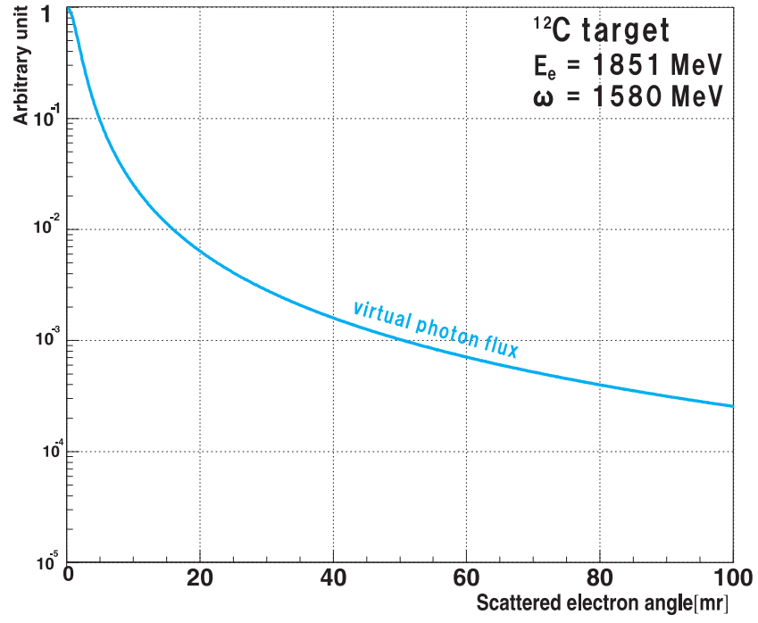
FIGURE 2.4: VIRTUAL PHOTON FLUX DEPENDENCE ON SCATTERED ELECTRON ANGLE FOR ^{12}\text{C} TARGET. PLOT IS OBTAINED WITH FOLLOWING KINEMATICS E_e = 1.851\text{GeV} AND \omega = 1.580\text{GeV} .
