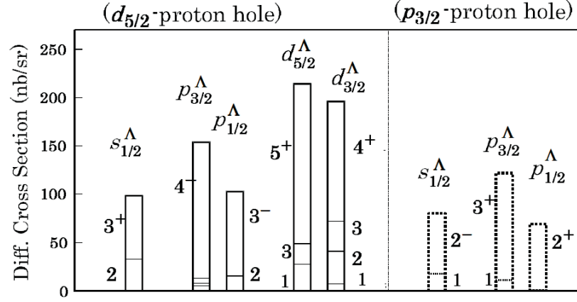
FIGURE 5.12: DIVIDED CONTRIBUTIONS TO THE PARTICLE-HOLE J-MULTIPLY STATE [j_p^{-1}j^\Lambda]_J FOR THE ^{28}\text{Si}(e, e'K^+)^{28}_\Lambda\text{Al} REACTION AT E_\gamma = 1.3 GEV AND \theta_{K^+}^{LAB} = 3^\circ WITH SLA MODEL. THE HEIGHT OF EACH PILLAR CORRESPONDS TO THE DIFFERENTIAL CROSS SECTION [99].
