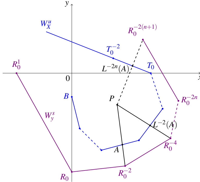
Figure 4.3: Proposition 4.2.3, case 1.1°.
