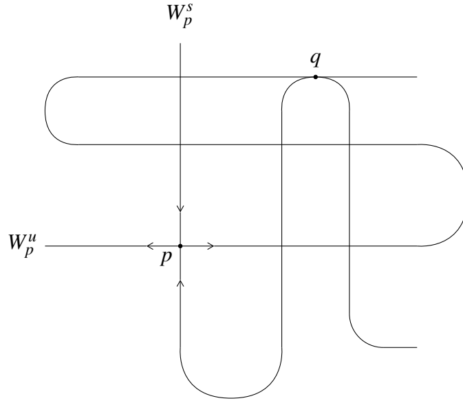
Figure 1.3: Point q is a tangential homoclinic point for p . All other points of intersection of W_p^s and W_p^s different from p on this picture are transversal homoclinic points.
