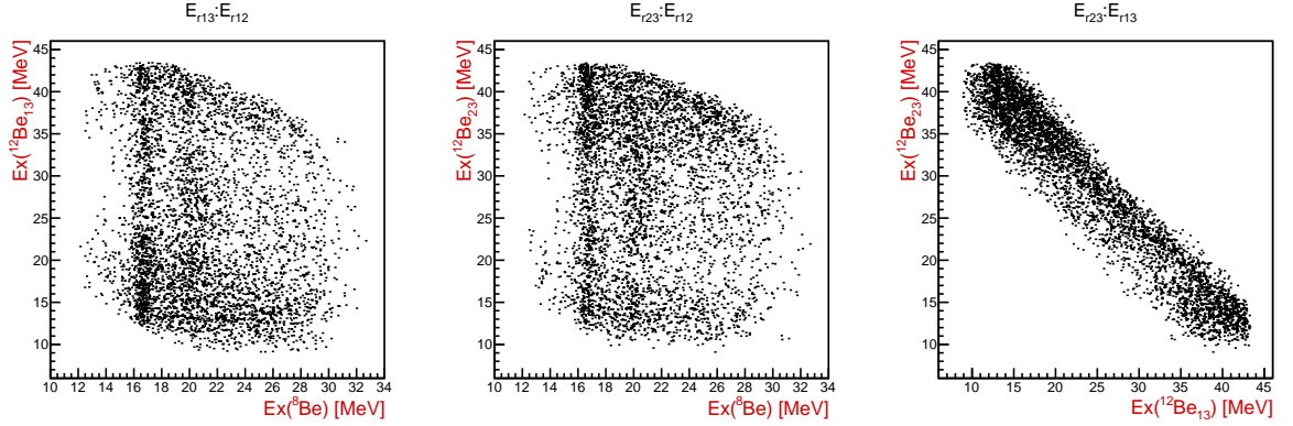
Figure 4.53: Excitation energy spectra for the ^8\text{Be}_{12}^{\text{nom.}} , ^{12}\text{Be}_{13} and ^{12}\text{Be}_{23} , from the ^7\text{Li}(^9\text{Li}, ^4\text{He}^4\text{He})_{\text{dT}=3}^8\text{He} reaction. Note that ^8\text{Be}_{12} excitation energy is calculated using nominal \Delta\phi_{12}^{\text{nom.}} = 180^\circ value.
