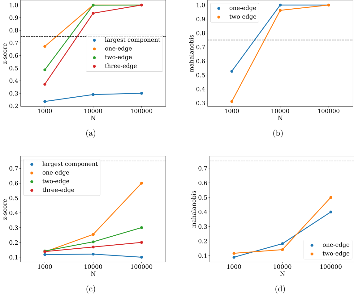
Figure 3.8: VM process results - scaled. We present the dependence of the percentage of significant ( p < 0.1 ) results for a voter model process with \langle k \rangle = 4 , fixed at 25% of the network default, on the size of the network. In panels a) and b) we show the one-tailed z-score and Mahalanobis distance results, respectively, for a voter model process with \zeta = 1 . In panels c) and d) we show the results when the parameter of the SI process is increased to \zeta = 10 . Horizontal lines are drawn at the limit in which 75% of simulations exhibit significant difference from the RRM-model.
