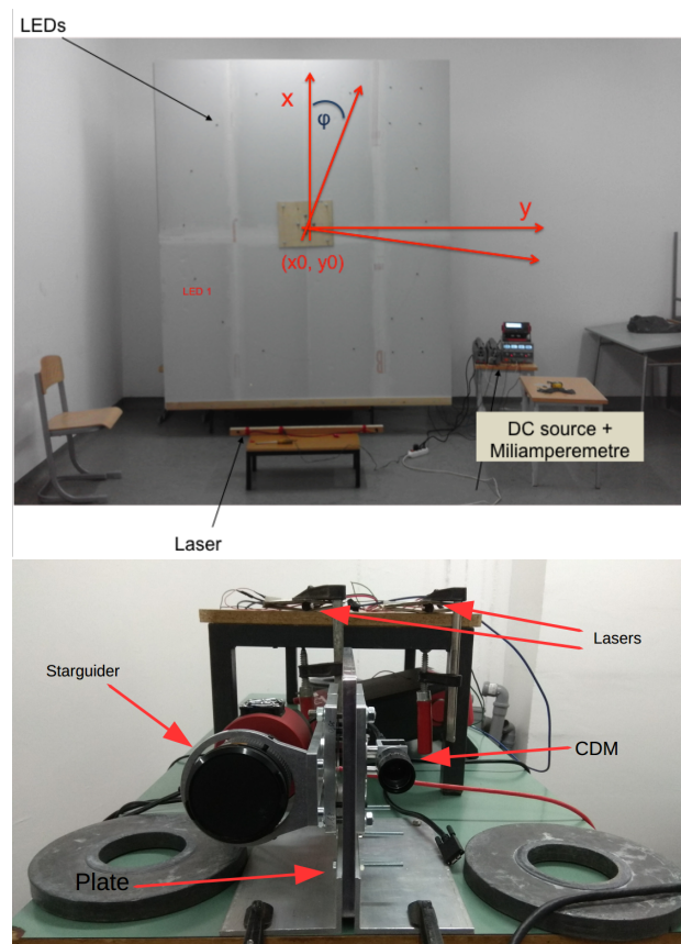
Figure 5.7: Setup in the laboratory. Top : 12 LEDs mounted on a circle of 2m diameter with the collimator holes of 1 mm. The whole board is mounted on a supporting plate which could be moved in steps of 0.02 mm and rotated in steps of 0.033^\circ . Bottom : Devices were setup on the other side of the lab, 20 m away, which included the CDM camera, SG camera and the reference lasers.
