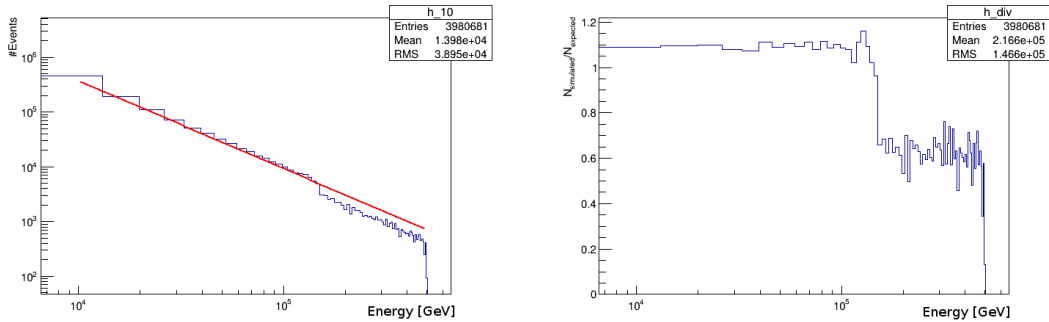
(a) Red line represents a power law with the slope of -1.6 with which the MCs were generated with. (b) This plot shows the ratio of the simulated and expected number of events from the power law with -1.6 slope.
