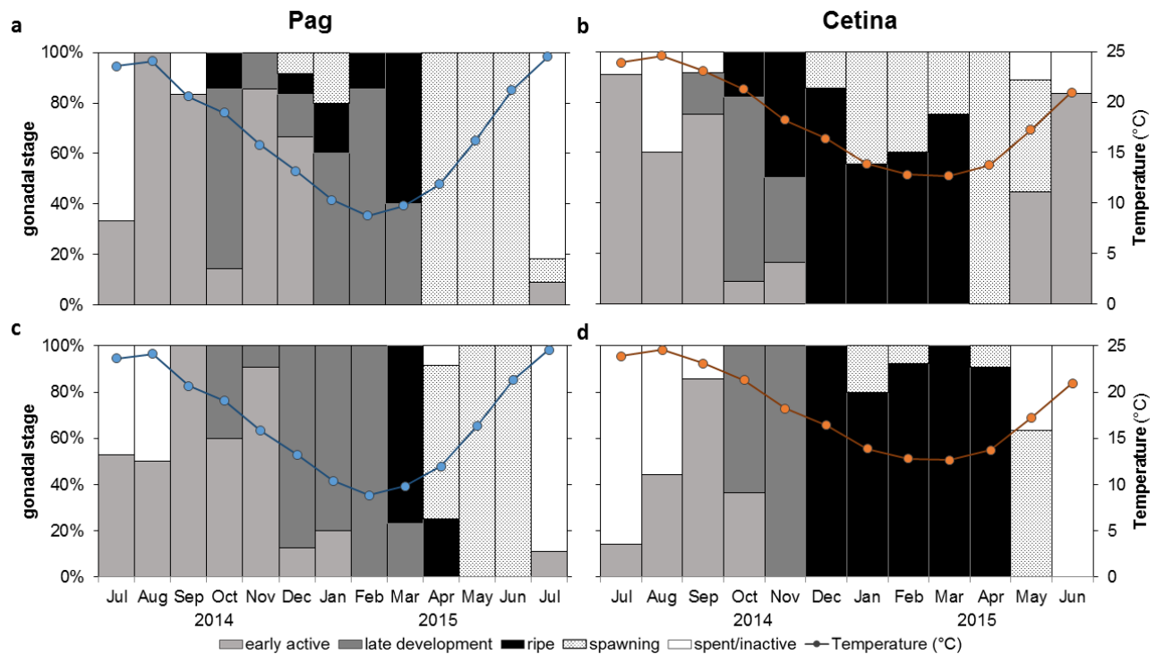
Figure 4.3.3. Monthly relative frequencies of gonad development stages of Callista chione and mean monthly temperature at Pag and Cetina sampling sites (a,b) females and (c,d) males.
