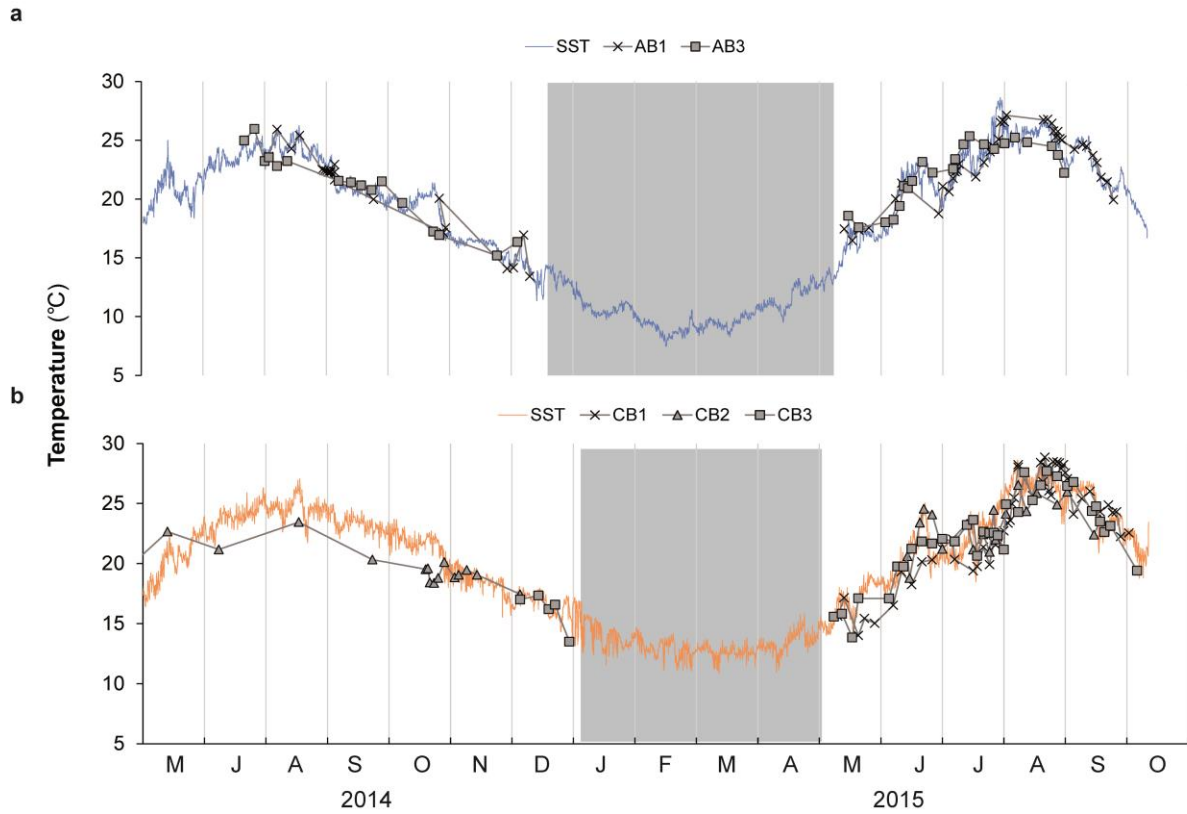
Figure 4.4.12. Temporal alignment of reconstructed \delta^{18}\text{O}_{\text{shell}} temperatures from instrumental SST in (a) Pag and (b) Cetina. Shaded area represents a period of slow/negligible growth.
