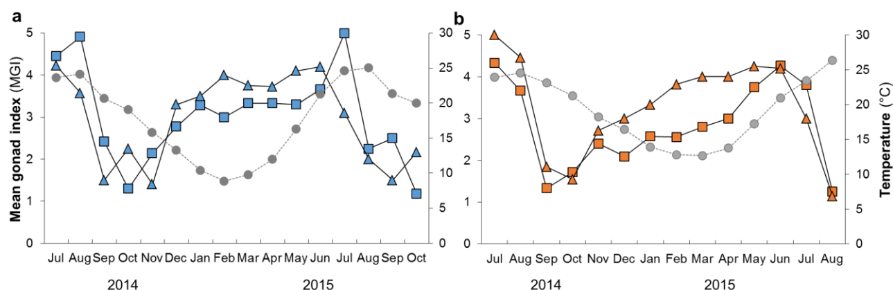
Figure 4.3.13. Mean monthly gonad index values of Glycymeris bimaculata and mean monthly temperature (circles); males (squares) and females (triangles) from (a) Pag and (b) Cetina.
