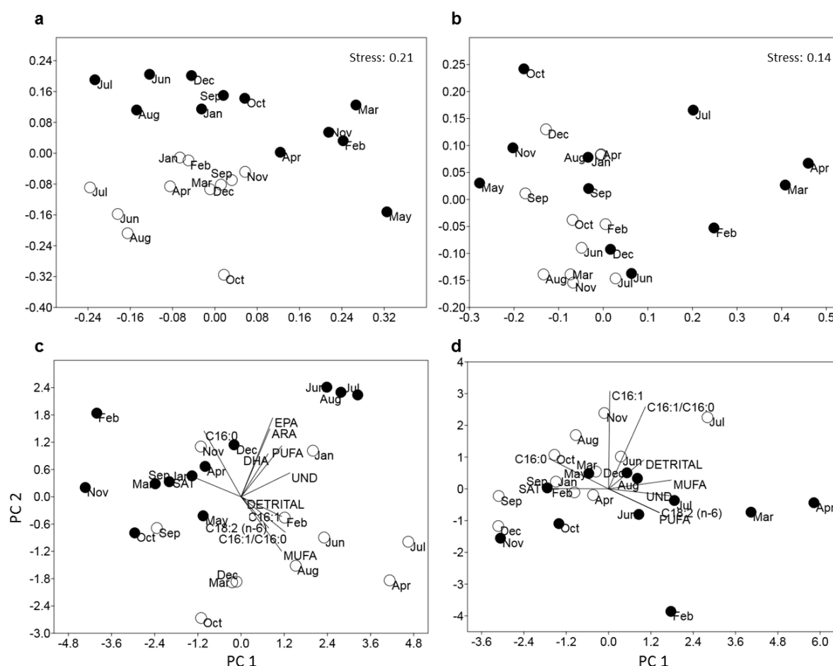
Figure 4.2.2. Above, non-metric multidimensional scaling (nMDS) of suspended particulate organic matter (SPM) (a) and sediment (Sed) (b) considering all FA profile means. Below, principal component analysis (PCA) output using most influential FA profiles in SPM (c) and Sed (d). Both sites are represented, Pag (filled) and Cetina (blank).
