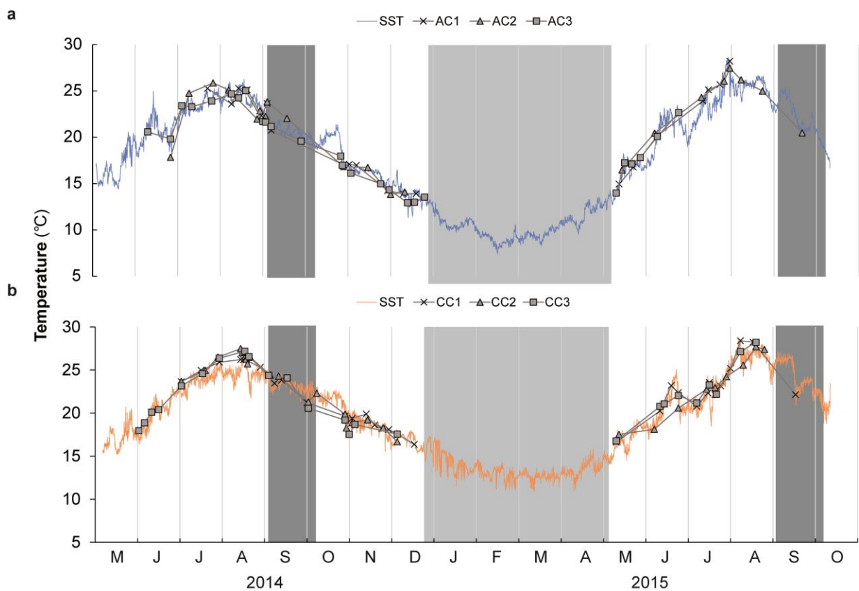
Figure 4.4.4. Temporal alignment of reconstructed \delta^{18}\text{O}_{\text{shell}} temperatures from instrumental SST in (a) Pag and (b) Cetina. Dark shaded area represents the approximate period of growth line formation. Light shaded area represents a period of slow/negligible growth.
