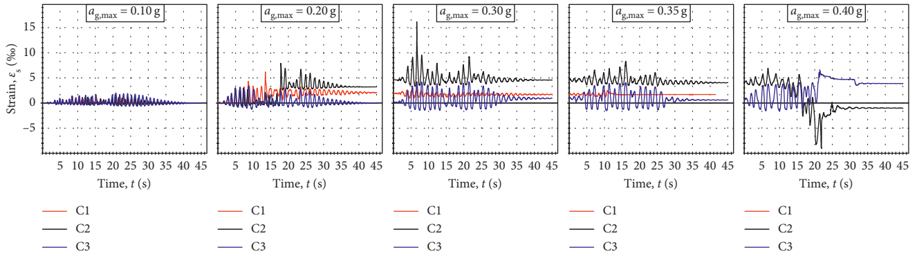
FIGURE 8: Reinforcement strain at the bottom of the column on the right side.
