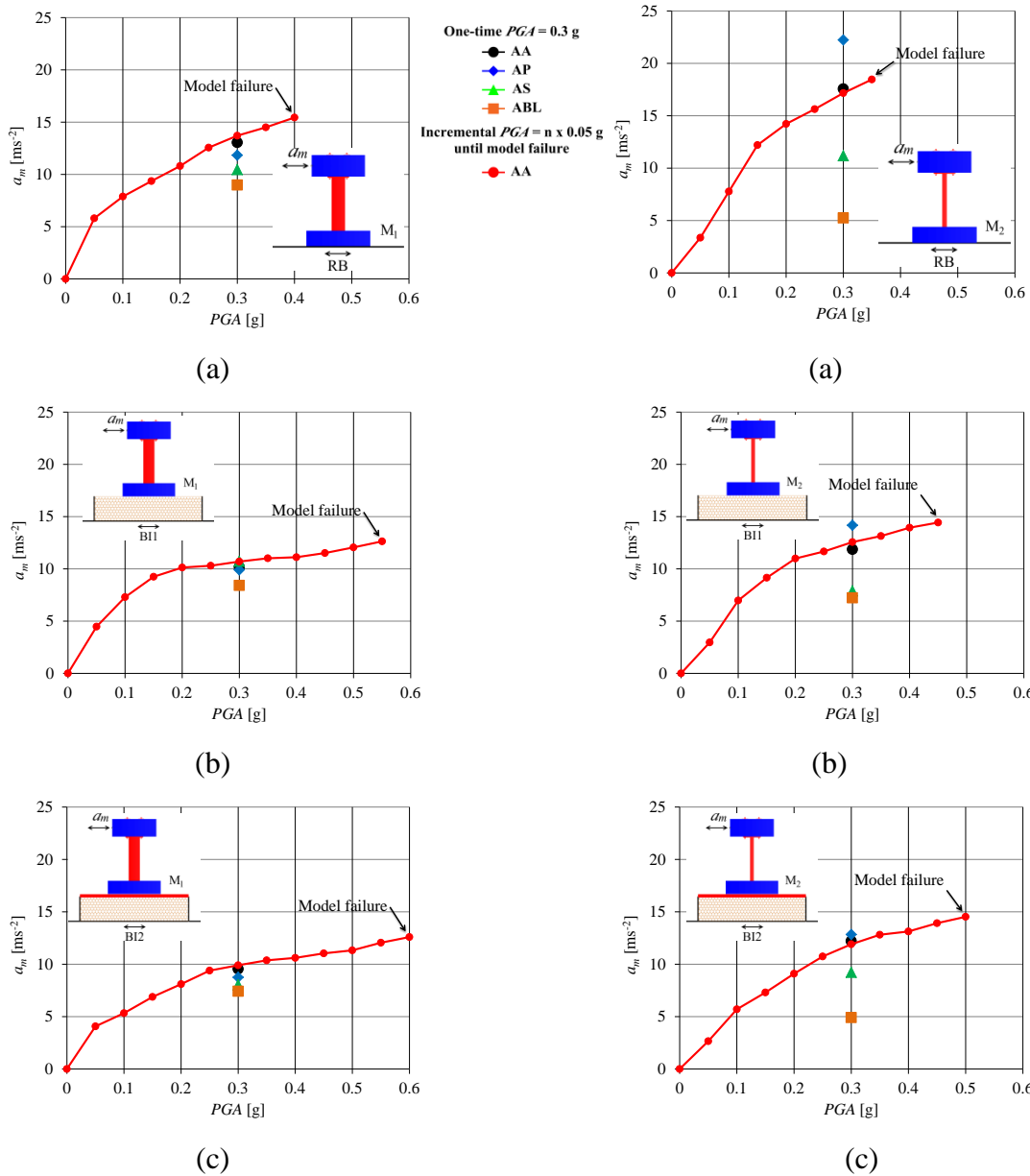
Figure 2.18 The peak acceleration a_m of the M_1 : (a) M_1 on RB; (b) M_1 on B11; (c) M_1 on B12
