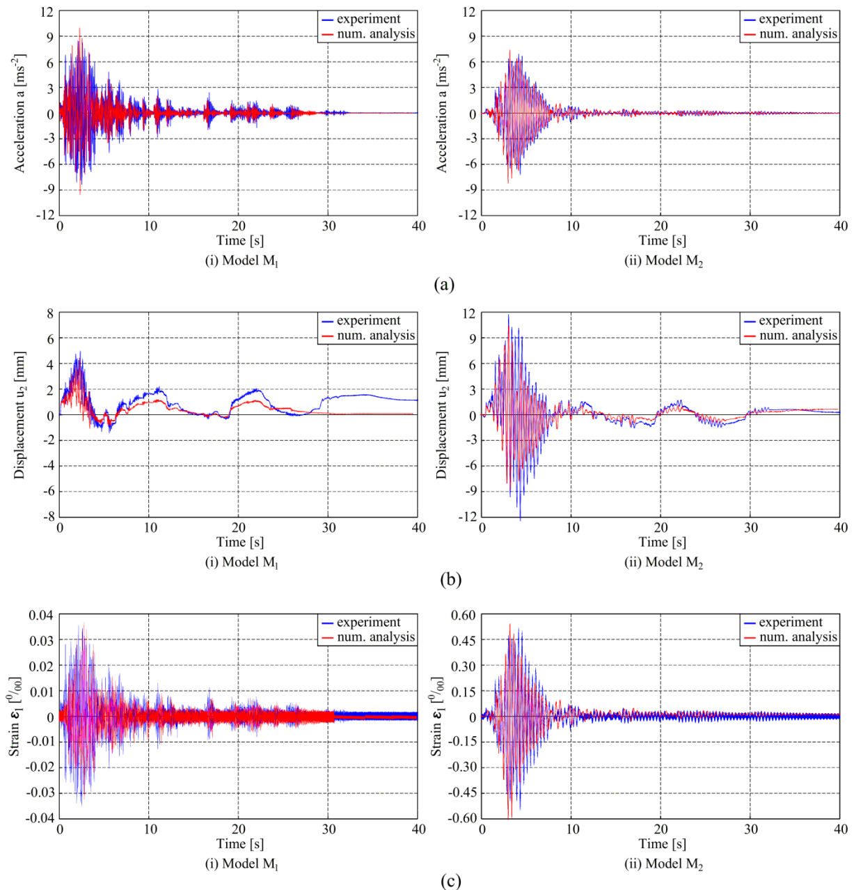
Figure 3.9. Comparison of experimentally determined and numerically obtained results for applied ABL accelerogram ( PGA = 0.3 g): (a) Horizontal acceleration a of the mass at the column top; (b) Horizontal displacement u_2 of the mass at the column top; (c) Vertical strain \varepsilon_1 on the right bottom side of the steel column
