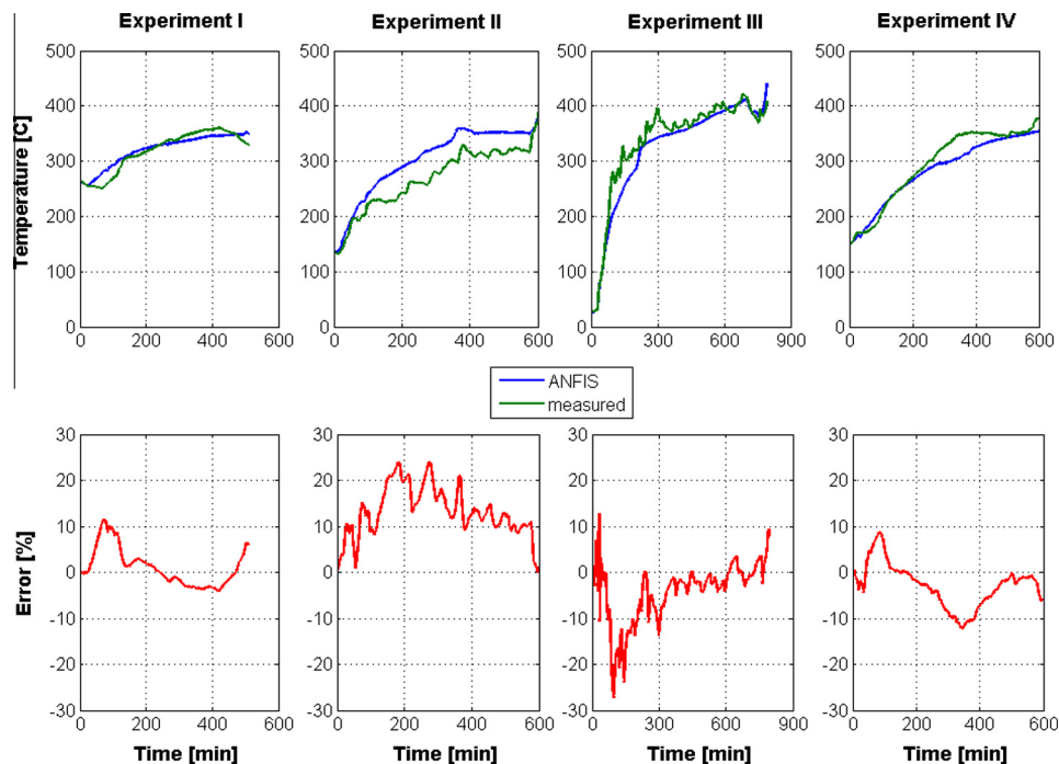
Fig. 8. Results of the neural network model for syngas temperature prediction – Pirna gasifier.
