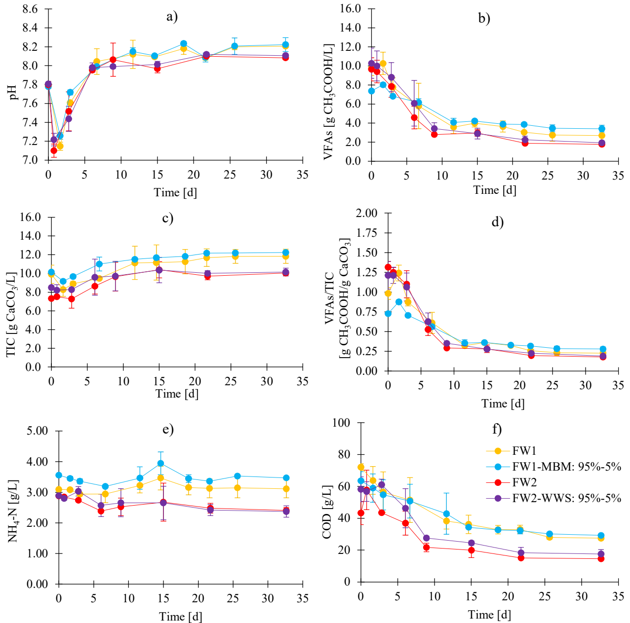
Figure 4 The change in variables in a liquid phase, a) pH, b) VFA, c) TIC, d) VFA/TIC, e) \text{NH}_4\text{-N} and f) COD during AD of selected mixtures
