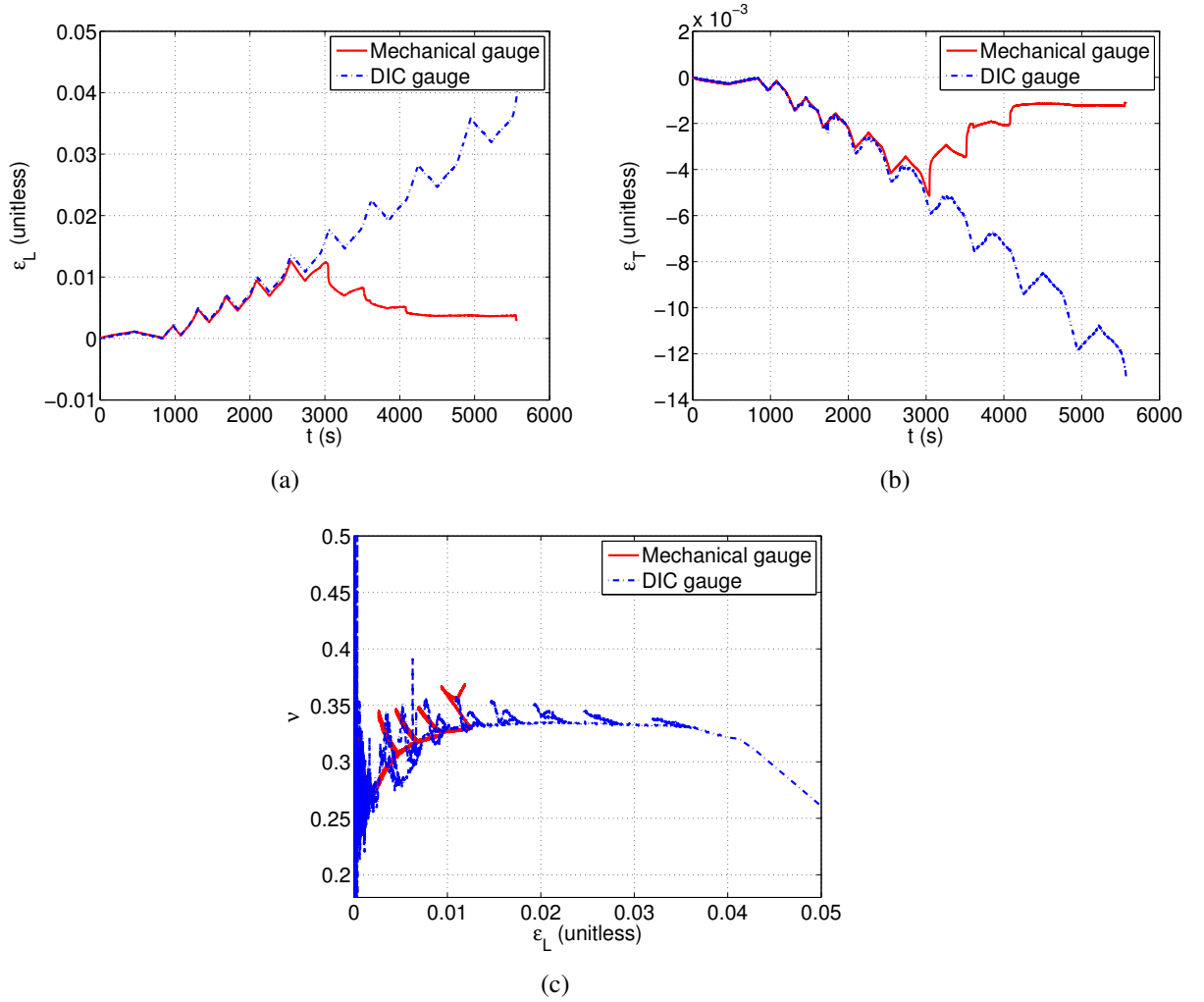
Figure 3.24: Comparison of measured \varepsilon_L (a) and \varepsilon_T (b) with strain gauge and DIC gauge. (c) Instantaneous Poisson's ratio calculated with Equation (3.1)
