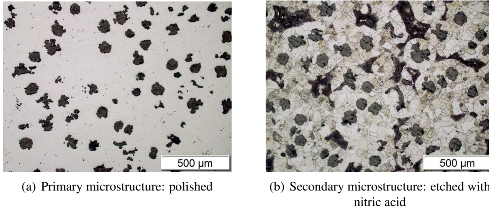
Figure 1.2: Metallography of flötret - type 200 SG cast iron [Čanžar et al., 2012]
