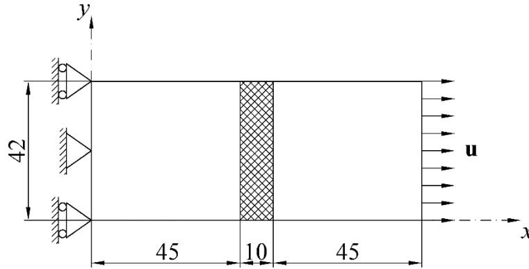
Figure 3.3 Geometry and boundary conditions of the plate subjected to tensile load. Based on [45].
