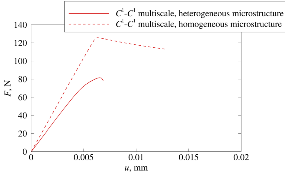
Figure 4.31 Structural responses of the plate subjected to compressive load obtained by the C^l - C^l multiscale scheme for homogeneous and heterogeneous microstructure
