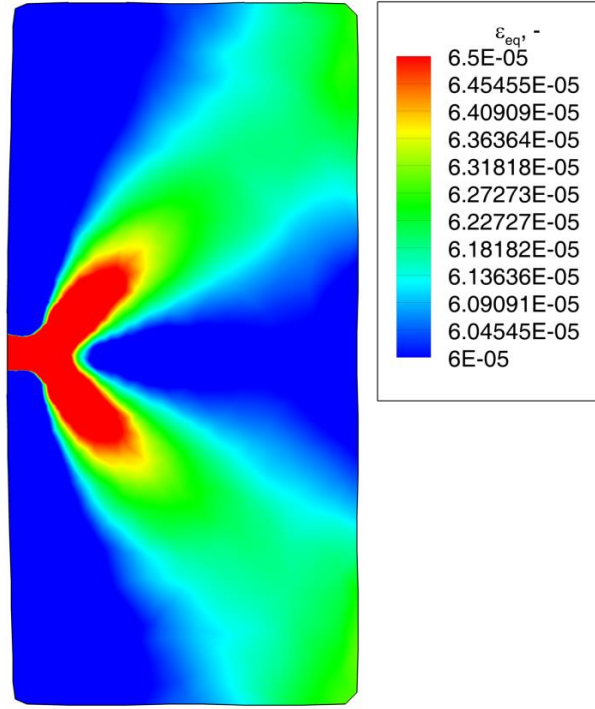
Figure 4.32 Distribution of the equivalent elastic strain \varepsilon_{eq} for heterogeneous microstructure with the internal length scale l_{micro} = 0.025 mm at the onset of softening
