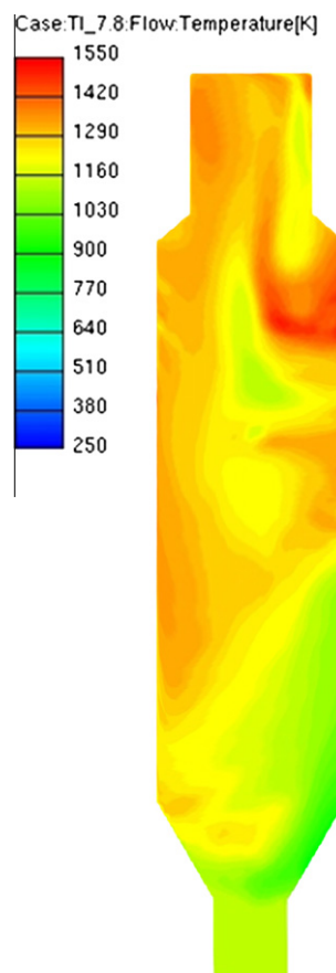
Fig. 8. Temperature field in vertical plane.
