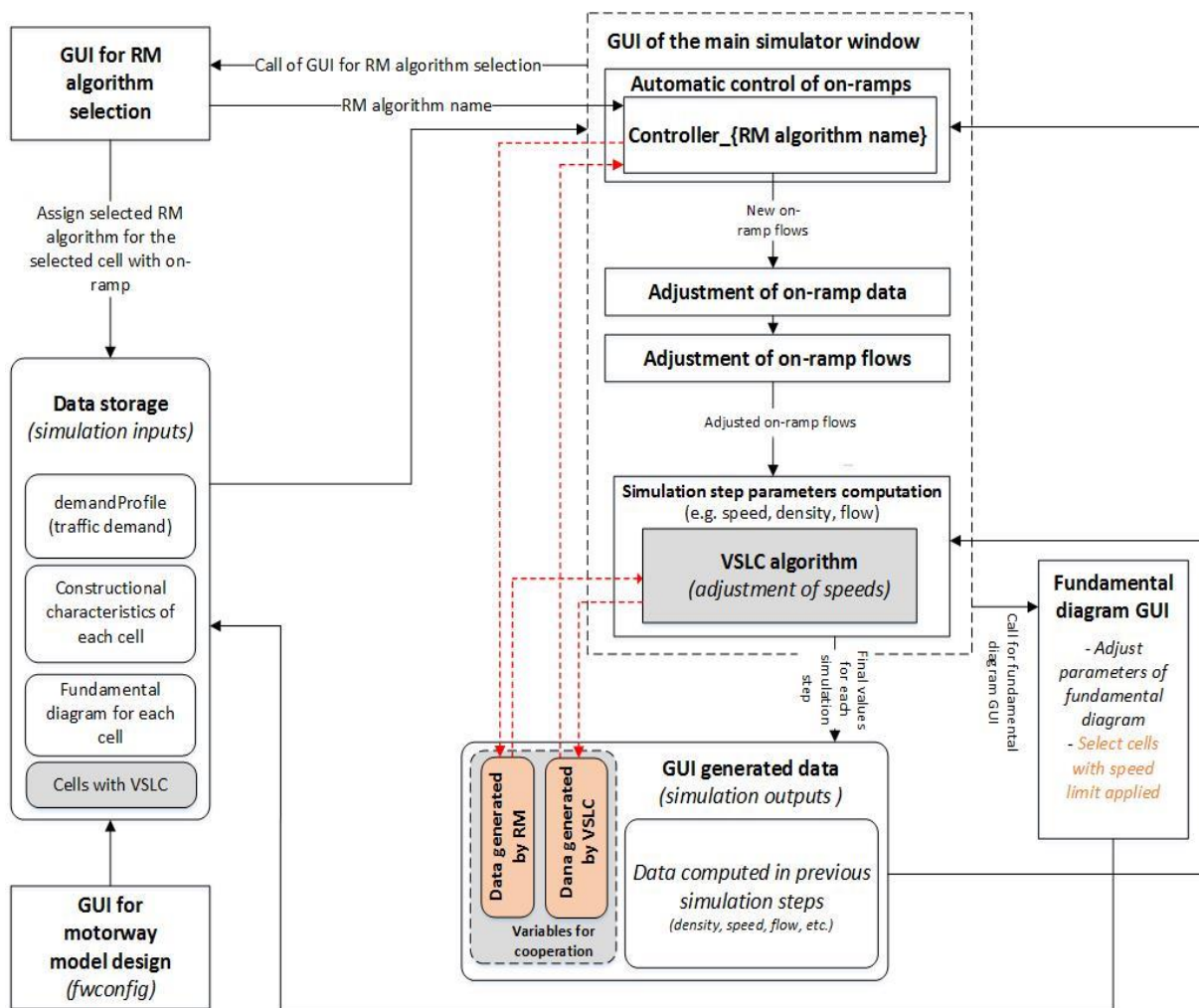
Figure 13: Position of variables that enable cooperation in CTMSIM software structure
