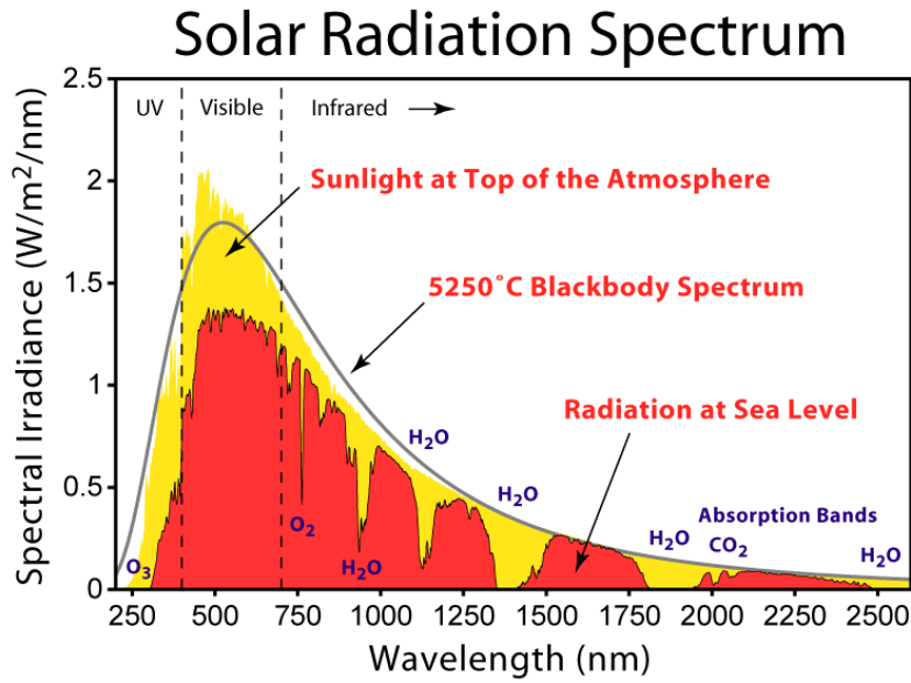
Figure 11: Solar radiation spectrum 3 (Licensed under CC BY-SA 3.0 via Wikimedia Commons)
