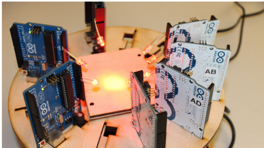
Figure 16: LED-to-LED communication testbed. Source: [134].
