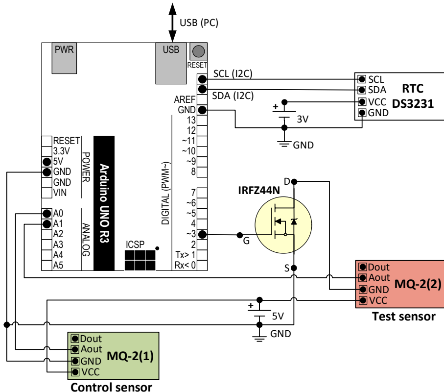
Figure 5.2. Setup scheme with the test and control sensors, and real-time clock for turning on and off the test sensor
