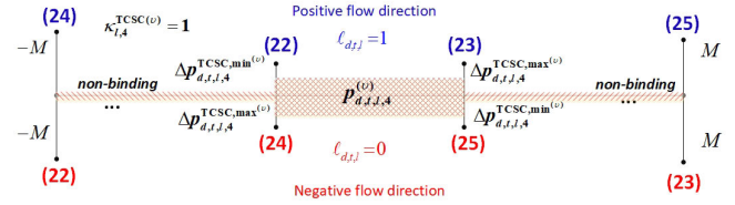
FIGURE 2. The explanations of TCSC constraints (22)–(25) on active power flow (e.g. if the compensation level 4 is installed).
