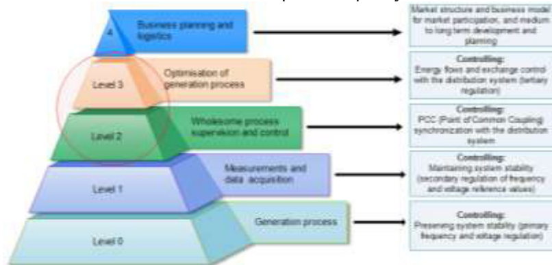
Fig. 2. IEC/ISA 95 standard hierarchy control adjusted for the observed microgrid concept
