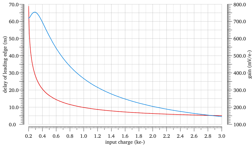
Figure 3.12: Simulated time-walk and gain curve for the front-end. The in-time threshold extracted from the red curve is 285\text{ e}^- .
