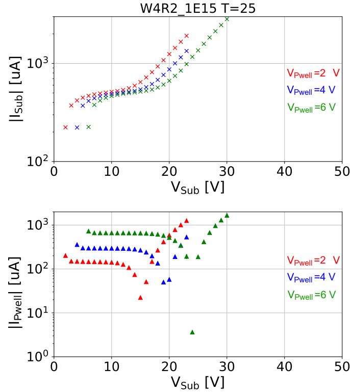
Figure 3.38: Sensor leakage current after neutron irradiation to 10^{15} \text{ n}_{eq}/\text{cm}^2 , measured at room temperature on the SUB and PWELL nodes with varying SUB voltage.
