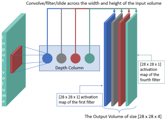
Figure 3.24: A graphical representation of a filtering sequence and building the output volume of activation maps
