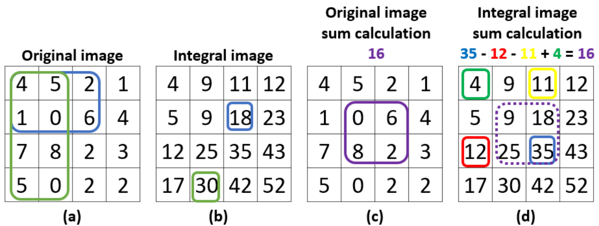
Figure 3.8: Original image (a), integral image (b), original image subregion sum calculation (c), and integral image subregion sum calculation (d)
