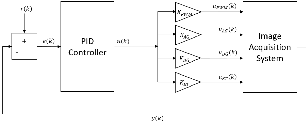
Figure 5.1: Simple split-range PID controller block scheme
