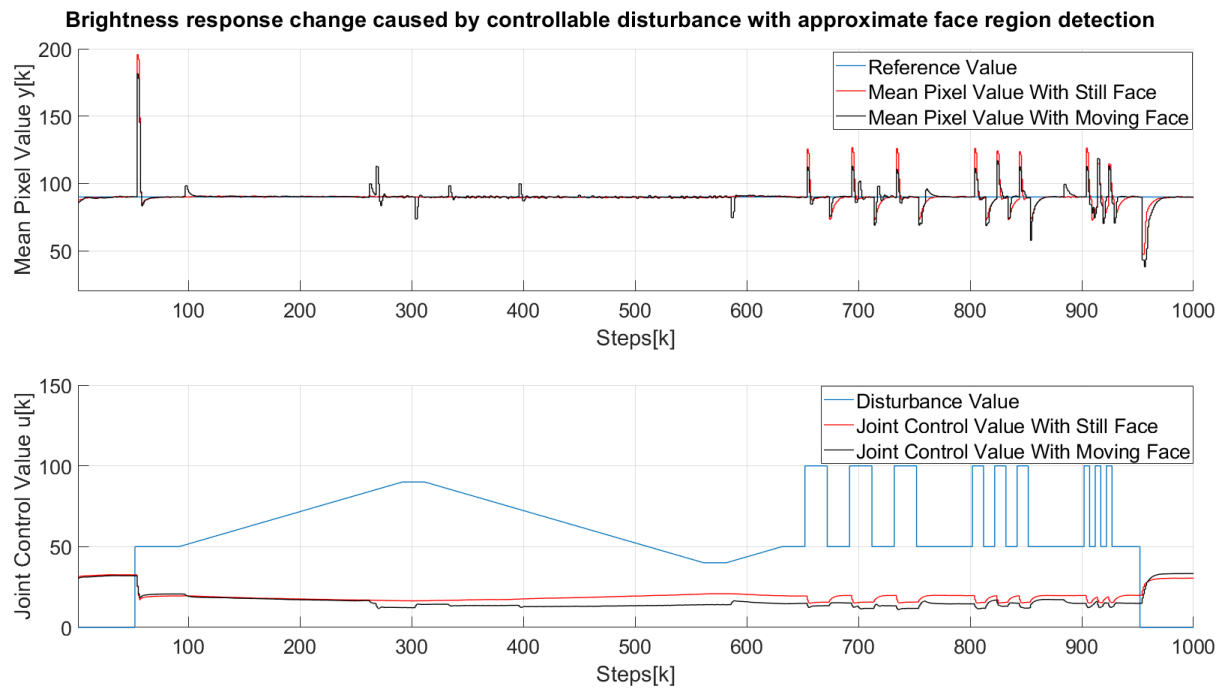
Figure 5.7: Brightness response change caused by a controllable disturbance with control and face region detection with a still and moving face
