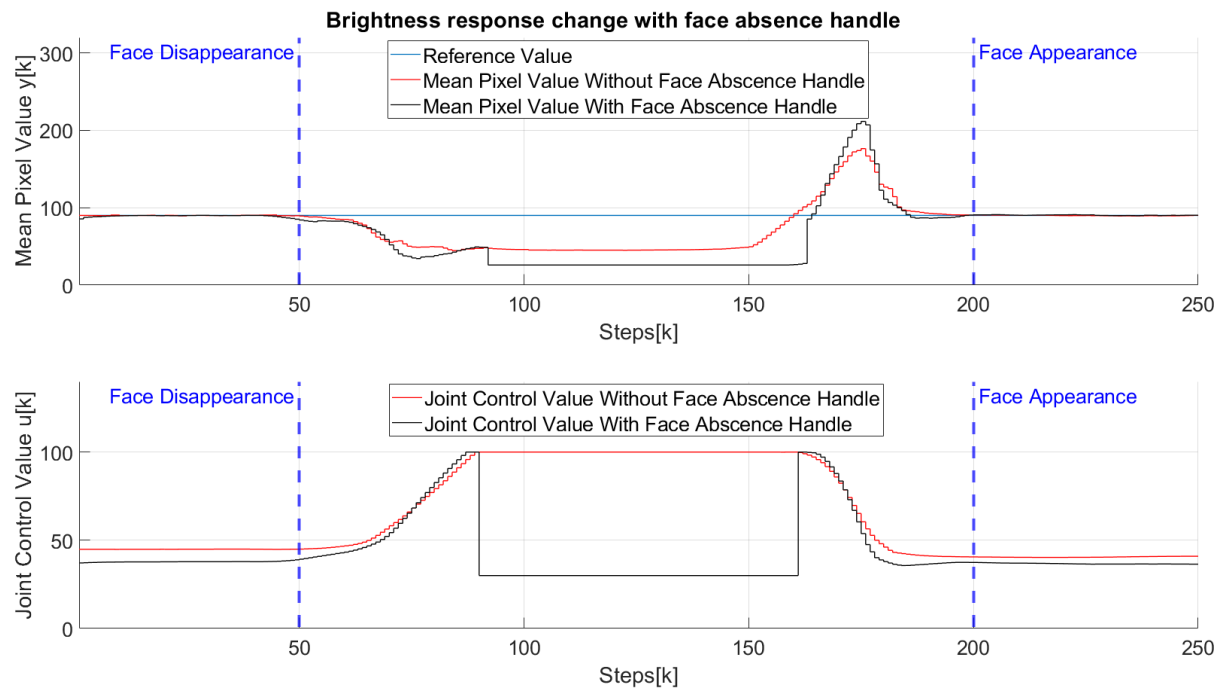
Figure 5.9: Face absence brightness response behavior without (red) and with (black) the face absence handle
