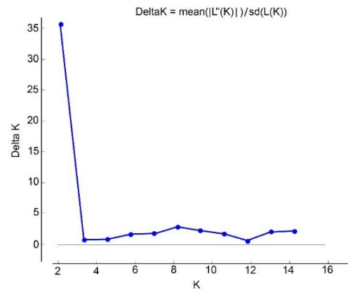
Figure 4. Results from Structure Harvester analysis reveal the most likely value of K based on STRUCTURE results.
